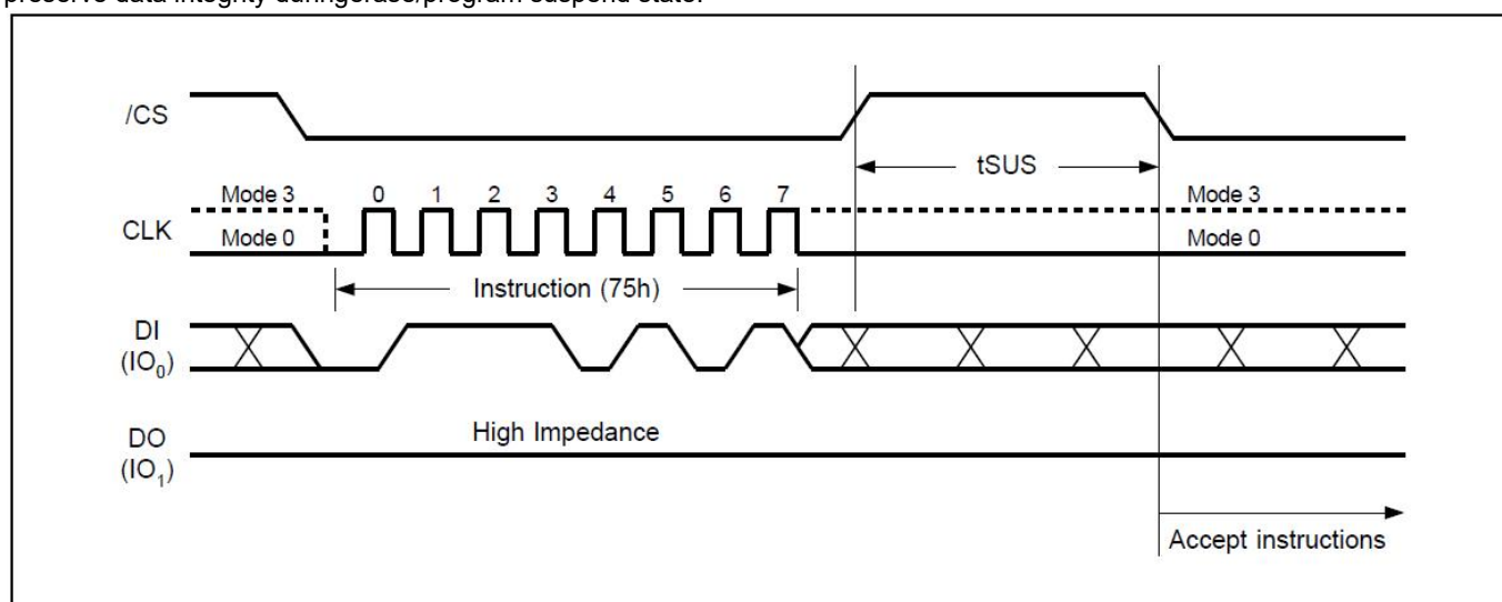
Figure 29a. Program/Erase Suspend Sequence Diagram for SPI Mode
