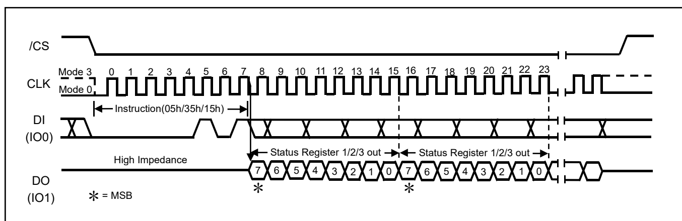
Figure4a. Read Status Register Sequence Diagram for SPI mode
