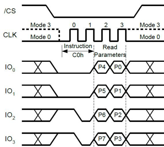
Figure 36. Set Read Parameters Instruction (QPI Mode only)
