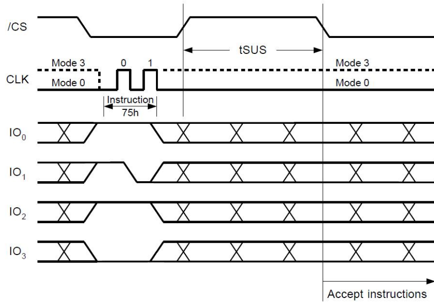
Figure 29b. Program/Erase Suspend Sequence Diagram for QPI Mode
