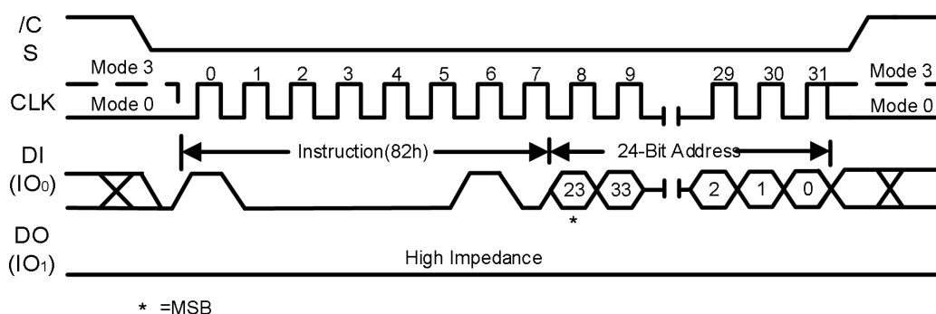
Figure 46. Mini Sector Erase Sequence Diagram
