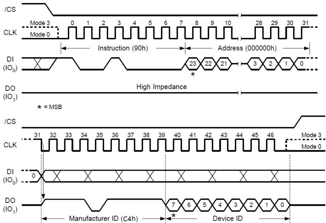
Figure 24. Read Manufacture ID/ Device ID Sequence Diagram for SPI Mode
