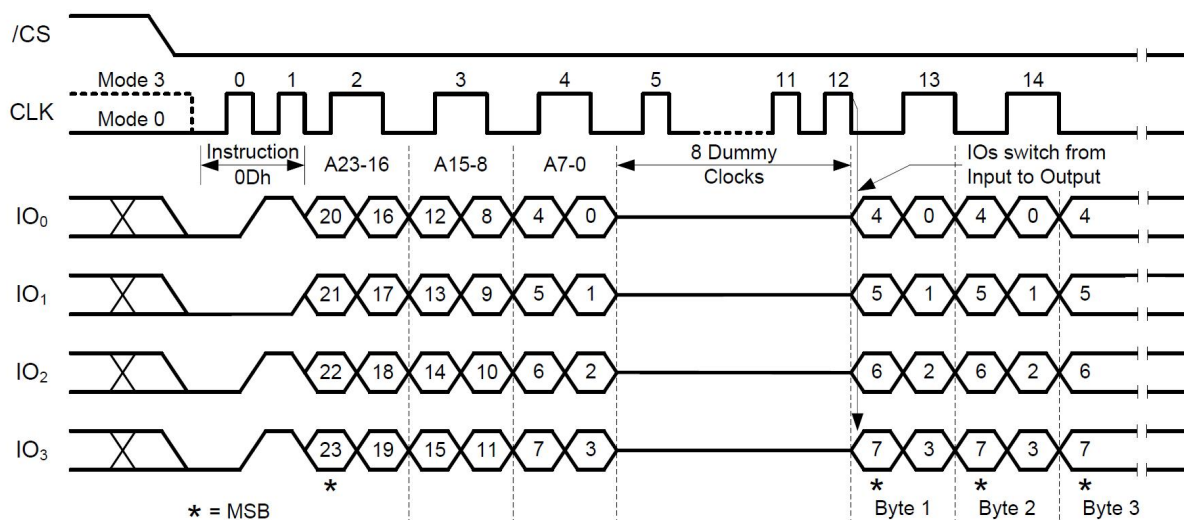
Figure 8b. DTR Fast Read Instruction (QPI Mode)
