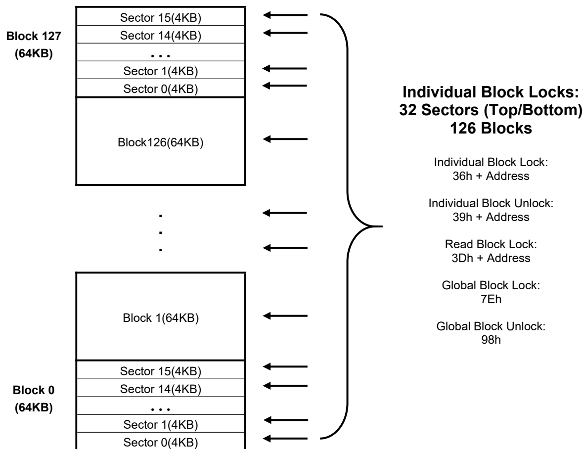
Individual Block/Sector Locks Figure IBL
